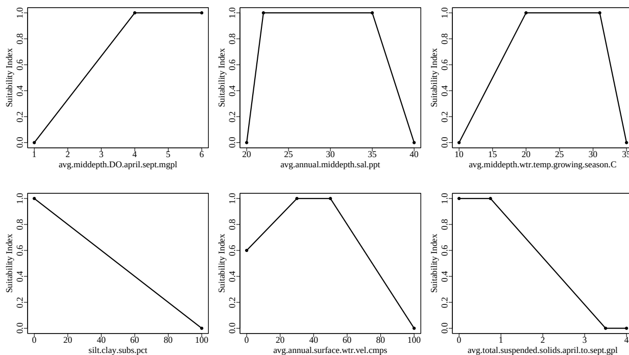
Figure 1. Suitability index graphs for variables included in the hardclam model in ecorest .
